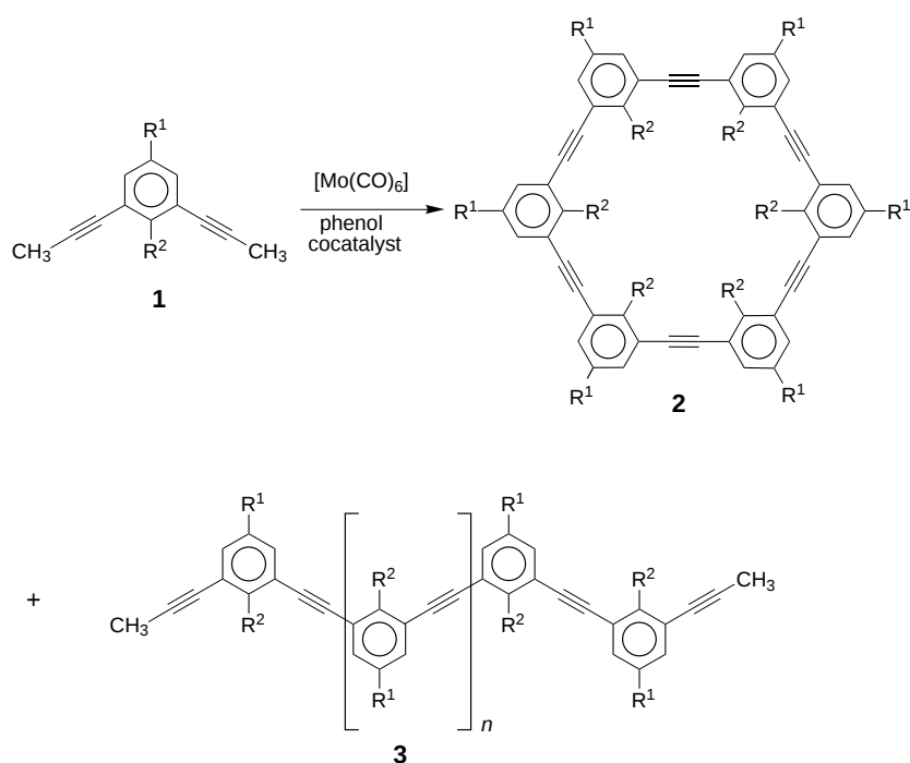
Scheme 1. Synthesis of 2 and 3 . Substituent pattern: a : \text{R}^1 = \text{tert-butyl} , \text{R}^2 = \text{H} ; b : \text{R}^1 = \text{hexyl} , \text{R}^2 = \text{H} ; c : \text{R}^1 = \text{dodecyl} , \text{R}^2 = \text{H} ; d : \text{R}^1 = \text{tert-butyl} , \text{R}^2 = \text{methyl} .
